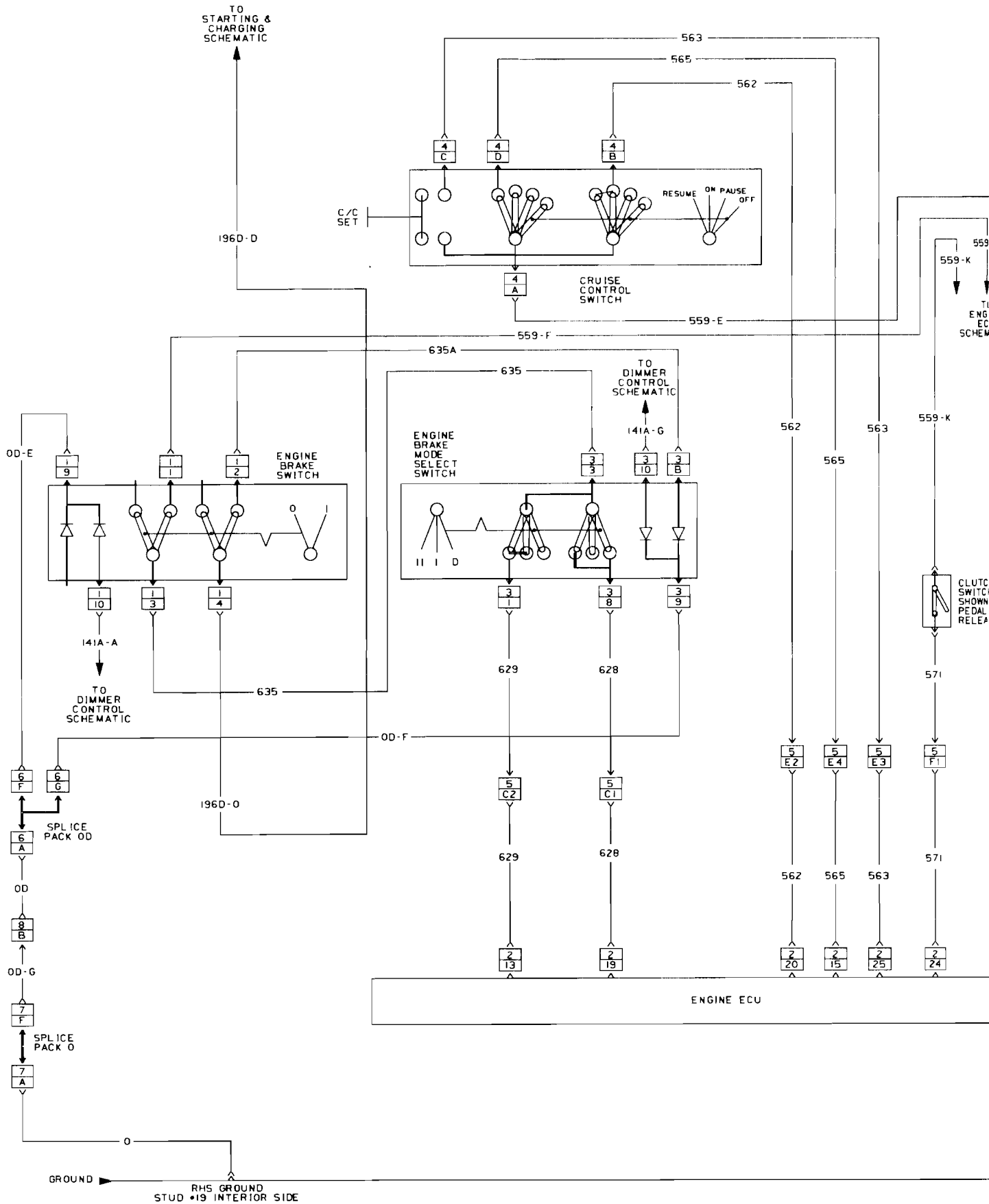
Engine Brake/CC/PTO, Caterpillar 3406E - VNL, VNM
