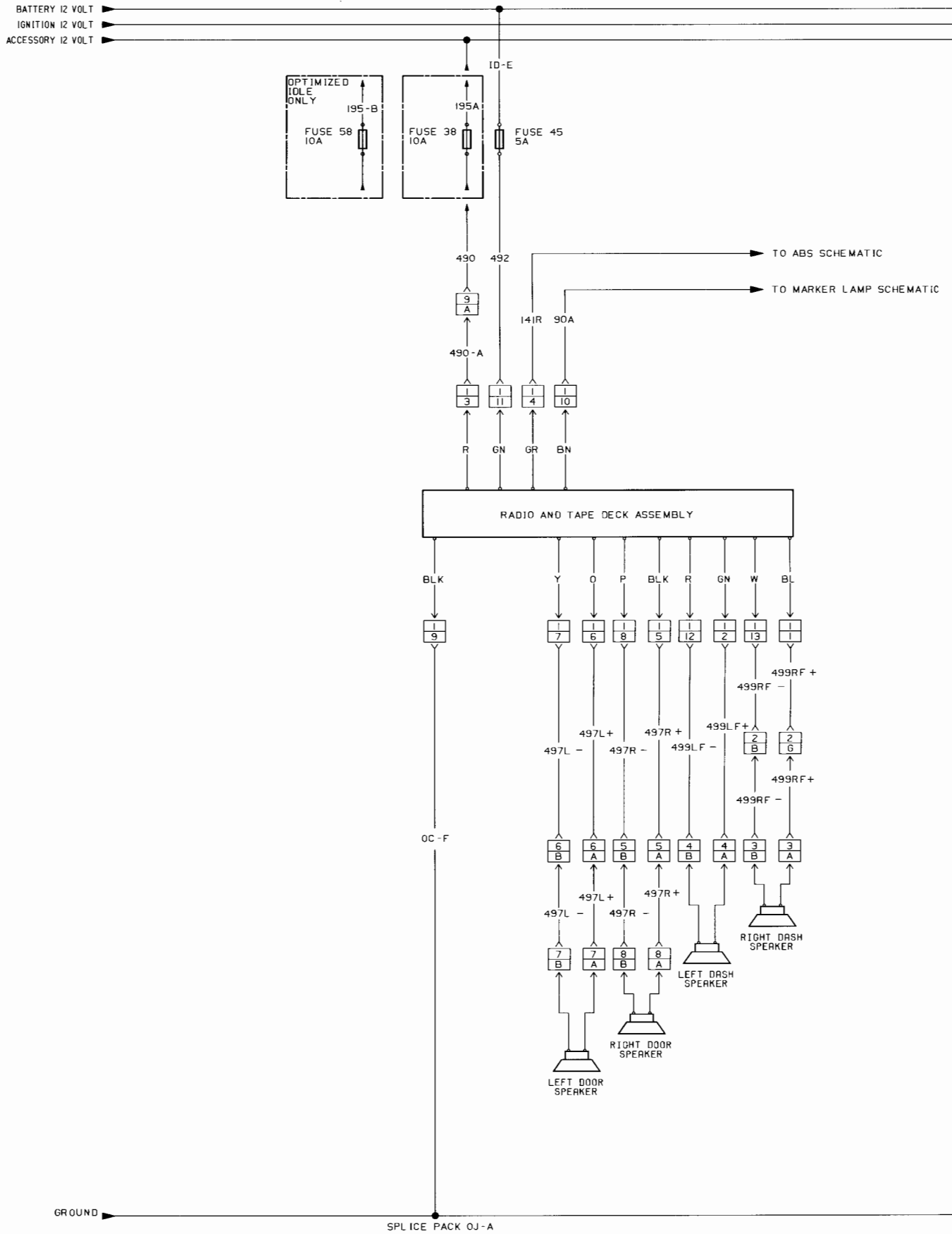
Radio in Dash, 4 Speakers - VNL, VNM
