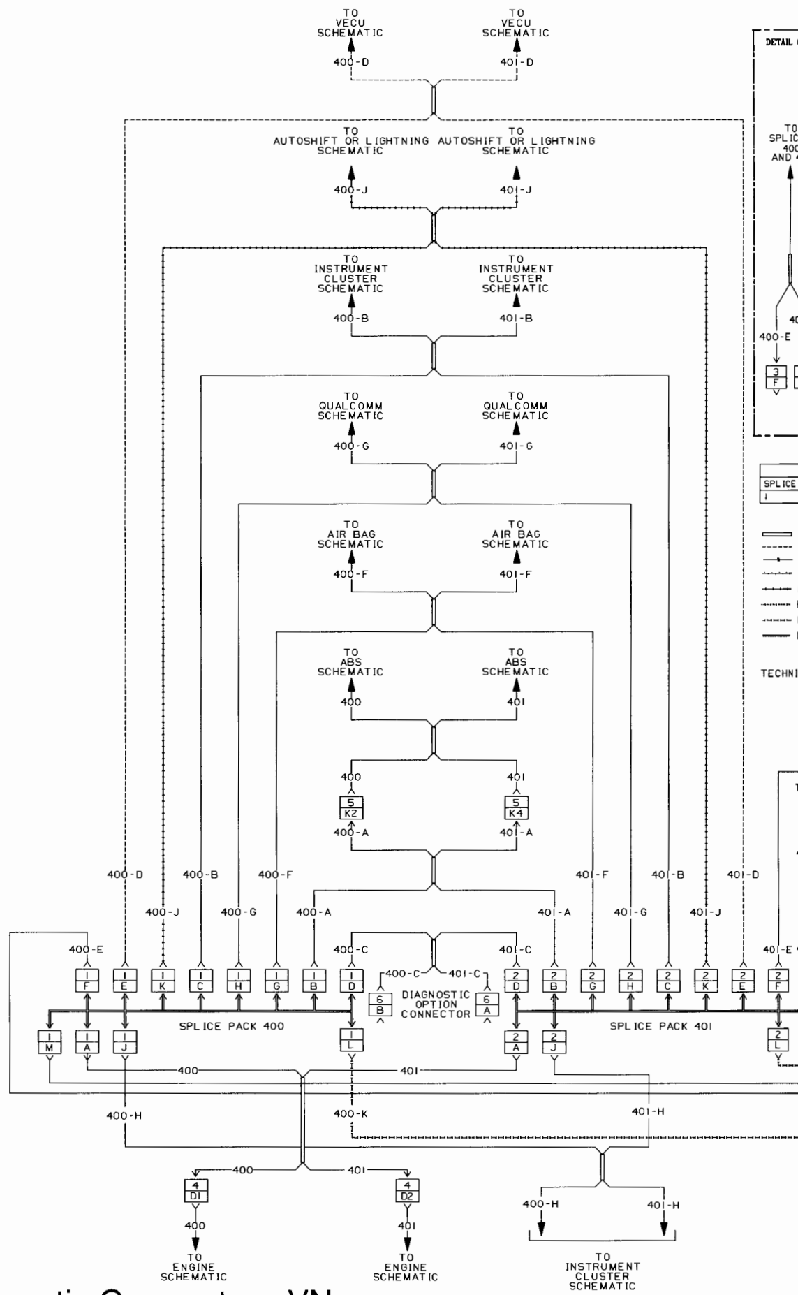
Data Link/Diagnostic Connector - VN
